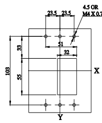
Knob cutout
